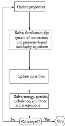
Pressure-Based Coupled Algorithm
