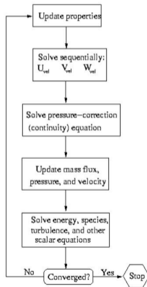
Pressure-Based Segregated Algorithm
